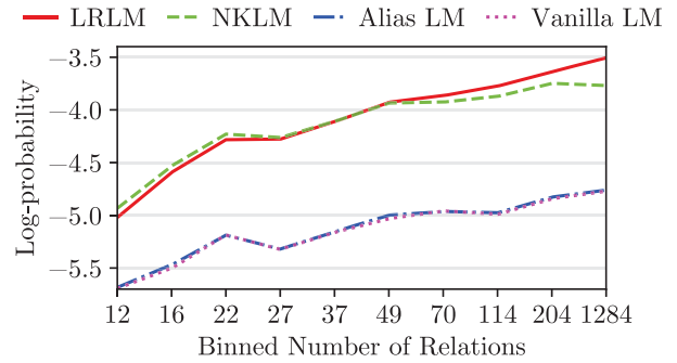
Figure 4: Word-average log-probabilities on development set of WikiFacts grouped by the average number of relations. LRLM shows a larger gain over the baselines as the number of relations increases.
