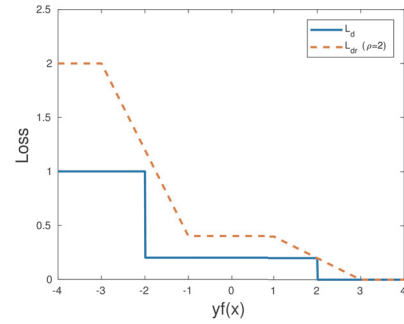
Figure 1: Double Ramp Loss with \rho = 2
