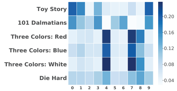
Figure 4: The attention visualization of memory networks.
