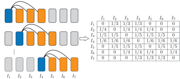
Figure 2: Item adjacent matrix construction example.
