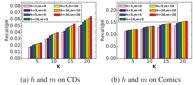
Figure 3: The variation of h and m .
