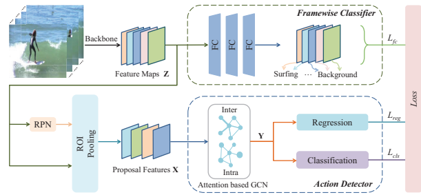
Figure 1: The architecture of P-3DCNNs embedded with our attention based GCN and framewise classifier modules. The model includes backbone subnet, RPN subnet, framewise classifier subnet and action detector subnet.
