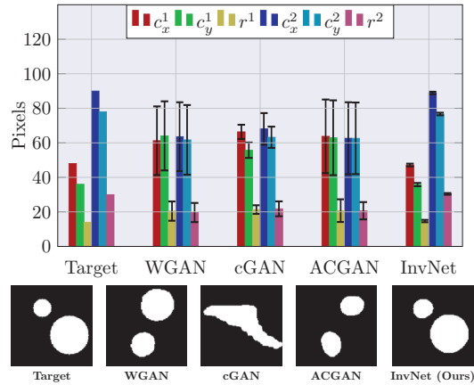
Figure 1: Examples from the manifold of images of two circles (with user-specified positions and radii) synthesized using various generative models. The bar/whisker plots show the accuracy of each model for respecting the specified invariances (center positions and radii for the i^{th} circle are represented by (c_x^i, c_y^i) and r^i respectively). WGAN provides no explicit control over the parameters of the generated circles, while cGAN and AC-GAN fail to generate satisfactory images. Our proposed InvNet model not only learns to reproduce correct shapes, but also provides effective user control over the location and size of the shapes. The large standard deviation for the properties show that the other approaches fail to learn the associated invariances.
