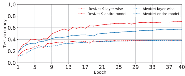
Figure 5: CIFAR-10 test accuracy for Adaptive Threshold.
