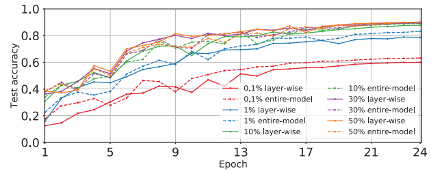
(b) ResNet-9
