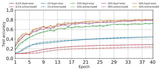
(a) AlexNet
