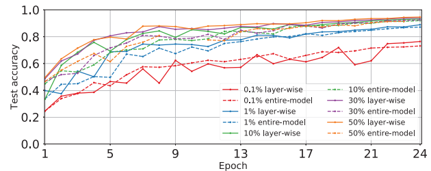
(c) ResNet-9 by using SGD with Nesterov’s momentum
