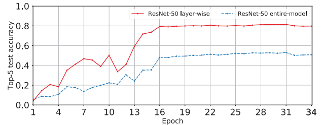
(b) ImageNet top-5 test accuracy
