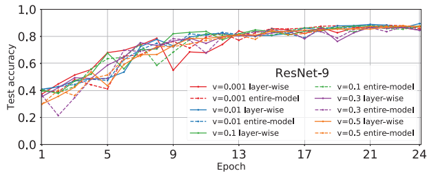
Figure 6: CIFAR-10 test accuracy for Threshold v compression.
