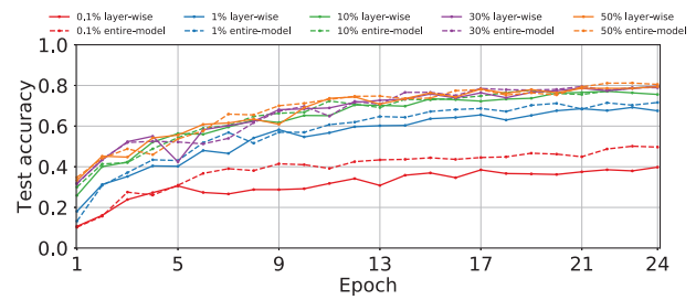
(a) AlexNet
