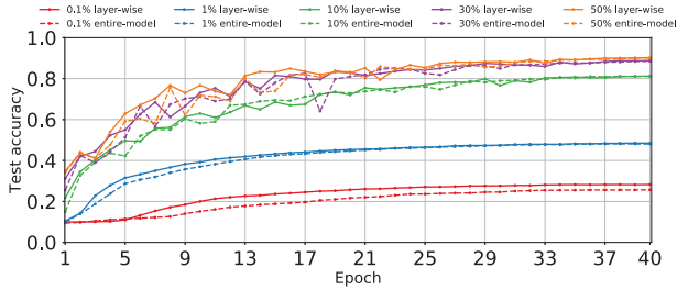
(b) ResNet-9
