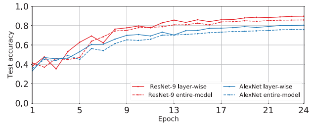
(a) CIFAR-10 test accuracy
