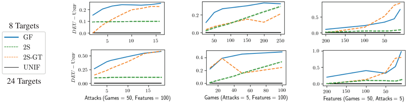
Figure 3: DEU – UNIF across the three strategies as we vary the number of features, number of training games and number of observed attacks per training game. When not varied, the parameter values are 100 features, 50 training games and 5 attacks per game. GF receives higher DEU than 2S for most parameter values.
