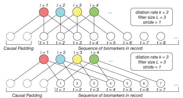
Figure 5: Dilated Convolutional Layers: given the EMR sequence, dilation rate k = 1 is a short-term standard convolution, and k = 2 means medium-term convolution skipping one record per input, and k = 3 means relative long-term convolution skipping two records
