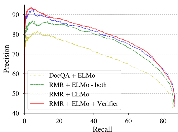
Figure 3: Precision-Recall curves of F1 score.
