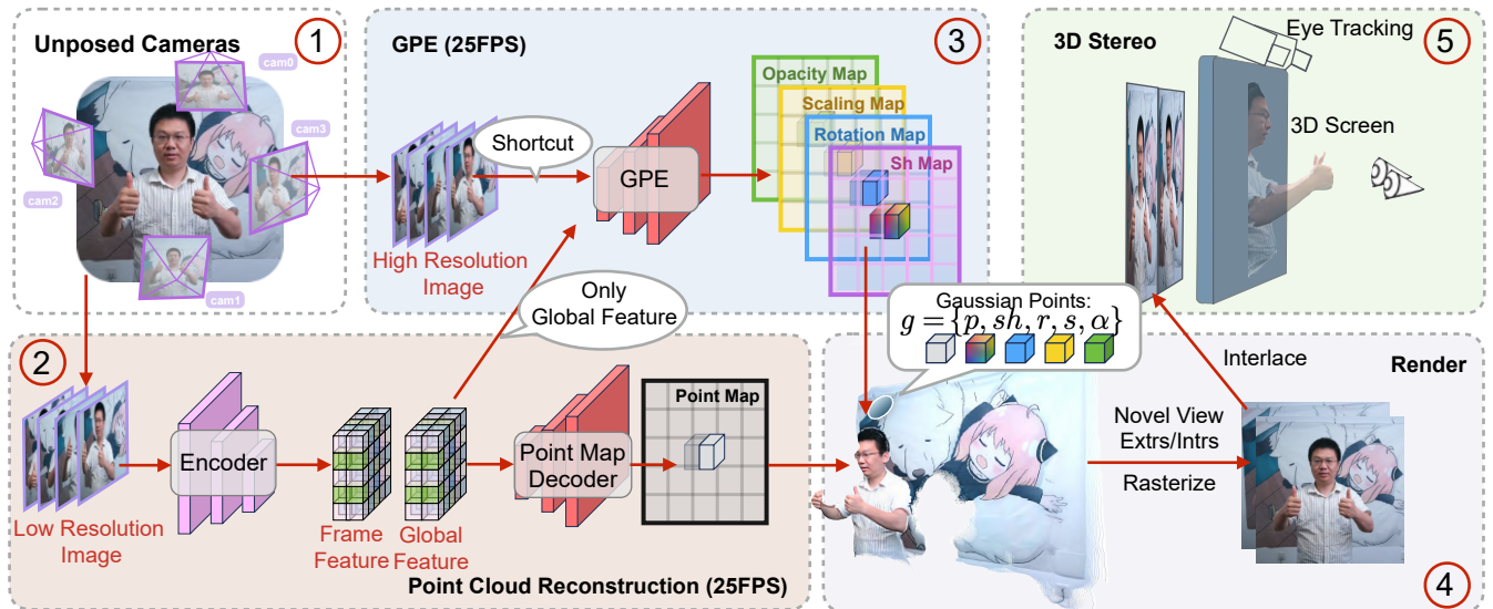
Figure 1: System architecture, illustrating how to achieve the 3D stereo from unposed cameras through steps 1 to 5.
