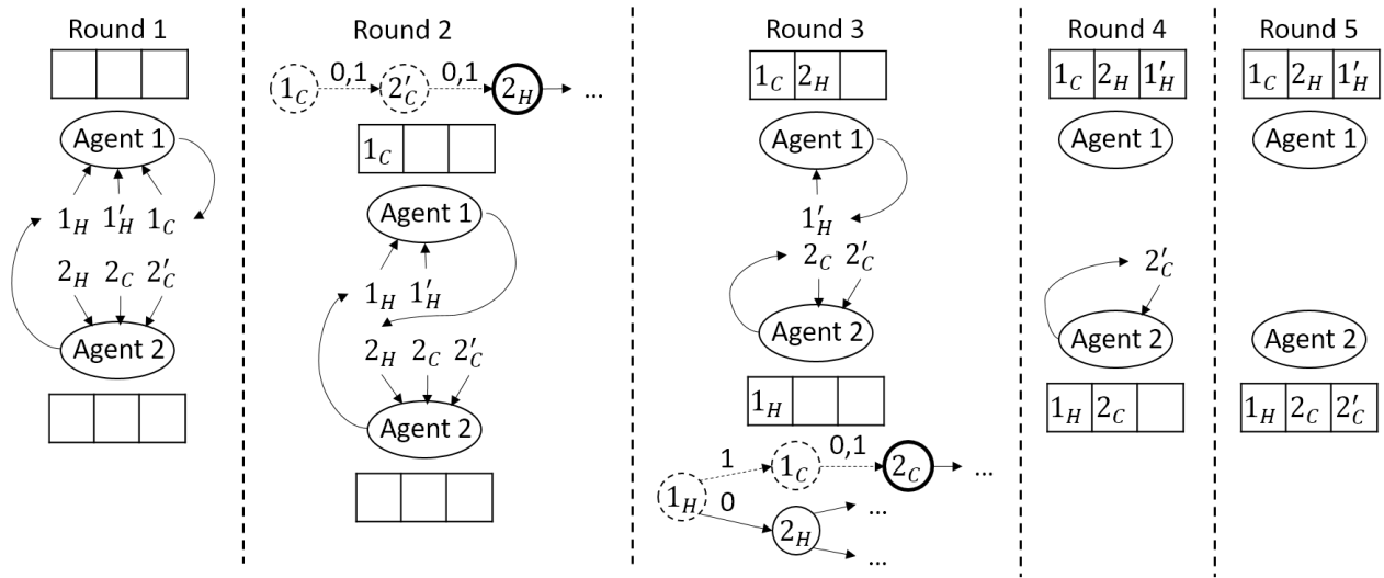
Figure 3: A run of TTC for the housing market from Example 1 and preferences in Figure 1.
