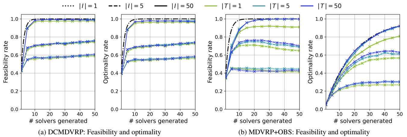
Figure 2: Feasibility and optimality rates on DCMDVRP and MDVRP+OBS across varying numbers of generated solvers, instances, and tests. The black dash-dot curve shows the rate under perfect selection i.e. the probability that at least one of the generated solvers is optimal.
