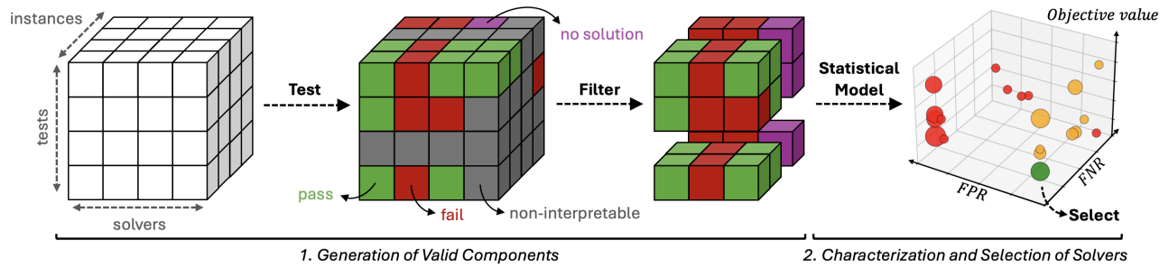
Figure 1: OptiHive produces optimization solvers through a two-stage process. In the first stage, it produces candidate solvers, problem instances, and tests, then filters out components to retain only fully interpretable solver-instance-test triples (represented as cubes). In the second stage, it applies latent class analysis to estimate the performance of each solver and selects the most promising candidate. Red, yellow, and green bubbles denote solvers that return non-interpretable or infeasible, feasible but suboptimal, and optimal solutions, respectively.
