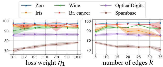
Figure 4: Parameter sensitivity on \eta_1 and k (DP %).
