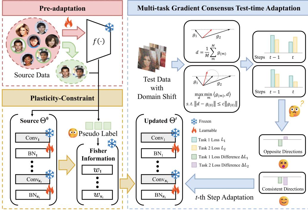
Figure 4: Our framework for MT-TTA. In the pre-adaptation phase, the model f is trained on the source domain to obtain the pre-trained parameters \Theta^0 . The pre-trained model generates pseudo labels corresponding to a random subset of source samples. The Fisher information matrix is computed for the plasticity constraint. During adaptation, the model explores the updated gradient space to find gradients that achieve a consensual direction on the loss difference \Delta\mathcal{L} , which are combined with the Fisher information to update \Theta^t jointly.
