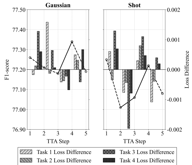
Figure 1: Experiments on CelebA with domain shifts of Gaussian and Shot noise. The X-axis denotes the test-time adaptation steps of performing M-TENT (Chatterjee et al. 2024) on tested samples. The figure shows a relationship between the relative change of task-specific loss (entropy) and F1 score on distribution shifts, i.e., consensual multi-task entropy reductions are likely to increase the performance while non-consensual ones might decrease the performance. An increase in performance is represented by a solid line, and a decrease is represented by a dashed line. The mixed positive and negative values of the bars indicate a conflict in the direction of the multi-task loss differences.
