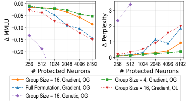
Figure 8: Locking robustness: performance of LLA-protected models under various attack and defense settings (averaged across 4 models).
