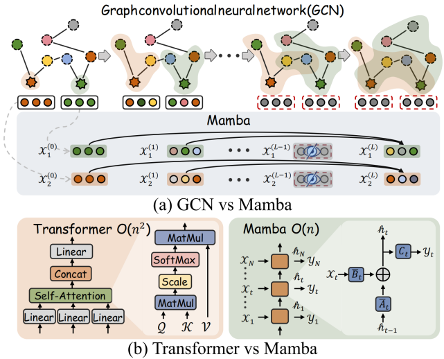
Figure 1: Comparison between GCN and Mamba (top), and comparison between Transformer and Mamba (bottom).
