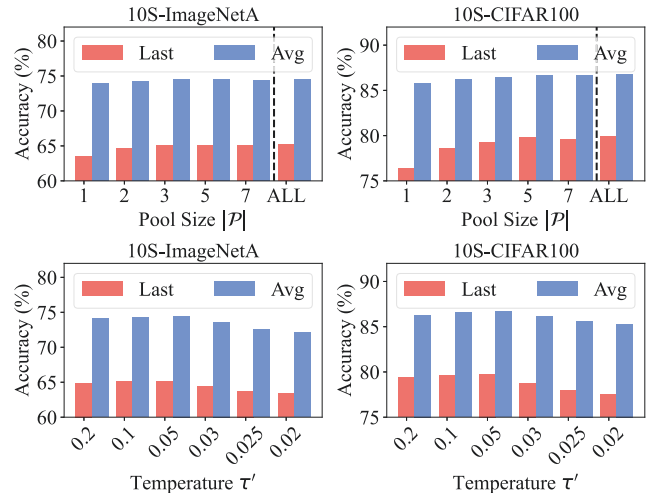
Figure 3: Model performances under different pool sizes |\mathcal{P}| and temperatures \tau' .
