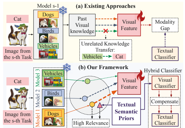
Figure 1: (a) Existing methods exhibit limited stability-plasticity trade-offs due to the unrelated transfer in backbone and the modality gap in classifier. (b) SECA leverage textual priors to (1) prioritize transferring relevant knowledge (Dog classes) when learning new classes (Cat), and (2) inject semantics into the visual classifier to bridge the modality gap.
