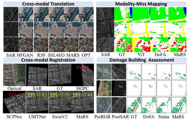
Figure 5: Visualization of the multi-modality VHR downstream tasks.
