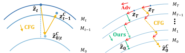
Figure 3: The proposed unconditional guidance corrects manifold deviation in DDIM denoising. The transition from z_t on manifold \mathcal{M}_t to z_{t-1} relies on predicting z_{0|t} . Left: CFG introduces a bias due to noisy signal interpolation, causing z_{t-1}^c to off-manifold. Right: The deviation introduced by CFG accumulates over denoising process, while our method provides internal guidance to ensure that each sampling points z_t remains on the valid manifold.
