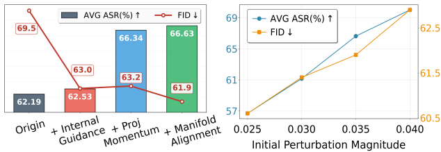
Figure 6: Ablation studies. Left: effectiveness of individual components; Right: Impact of initial perturbation magnitude. Sensitivity analysis for key hyperparams (reconstruction starting point, momentum coefficient) in Appendix D.
