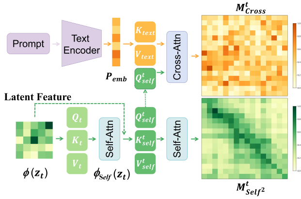
Figure 4: Architectural Comparison for Adversarial Guidance. Top: Standard cross-attention fuses static, external text embeddings P_{\text{emb}} with image features, leading to potentially noisy and unstructured guidance maps M_{\text{cross}}^t ; Bottom: Our cascaded self-attention ( \text{SA}^2 ) generates a highly structured guidance map ( M_{\text{self}^2}^t ) based solely on time-varying internal features derived from the current noised latent z_t , providing a stable, semantically-consistent guidance signal \epsilon_{\theta}^I (More visualizations in Appendix E).
