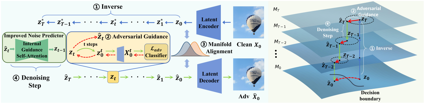
Figure 2: Overview of the proposed HAM framework. (1) Inversion: A high-fidelity inverse trajectory \{z_t^*\}_{t=0}^T is first derived from the clean image using a high-order ODE solver; (2) Adversarial Guidance: At each timestep t , an adversarial gradient is computed using the current latent z_t . This gradient is then projected onto the manifold to create a raw adversarial push \delta_t ; (3) Manifold Alignment: The perturbed latent \hat{z}_t = z_t + \delta_t is dynamically aligned with its clean reference z_t^* by matching their statistical properties (mean and variance), resulting in the final aligned latent \hat{z}_t ; (4) Denoising Step: A prompt-free, self-attention-guided denoising step is performed on \hat{z}_t to compute the latent for the next timestep z_{t-1} and ensure structural consistency, which repeats until the adversarial image is generated.
