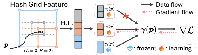
Figure 2: Illustration of the proposed coarse-to-fine hash encoding strategy. Given any input coordinate \mathbf{p} , the low-frequency feature (i.e., \gamma_1 ) is learned first and then frozen. As the optimization proceeds, higher-frequency features (i.e., \gamma_2 and \gamma_3 ) are progressively optimized.
