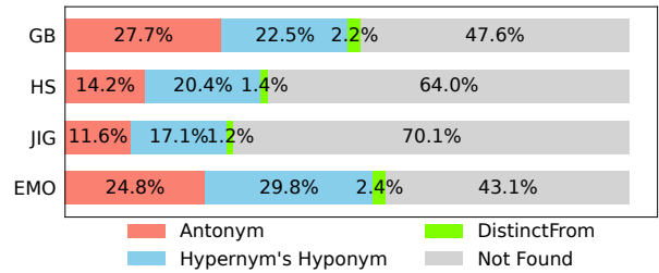
Figure 5: Categories of words returned from ConceptNet.
