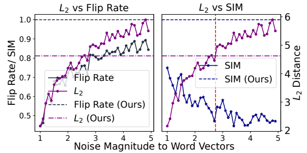
Figure 3: Trade-off between L_2 distance between word embeddings of original and perturbed token versus Flip Rate—i.e., the chance of perturbed token converting to the new word, and context similarity (SIM) on DistilBERT with JIG dataset.
