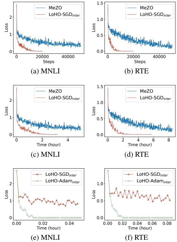
Figure 5: Convergence rate comparison on RoBERTa-large.
