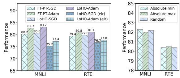
Figure 3: Ablation study of hybrid optimization.
