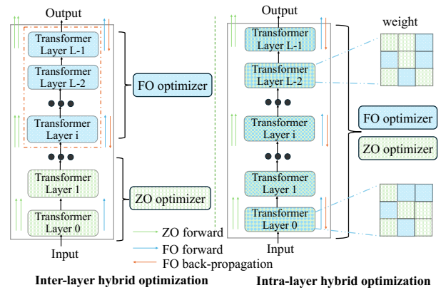
Figure 1: Low-order Hybrid Optimizer (LoHO).
