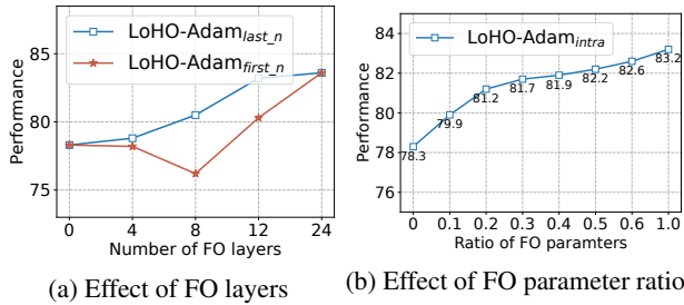
Figure 4: Effect of FO layers and the ratio of FO parameters.
