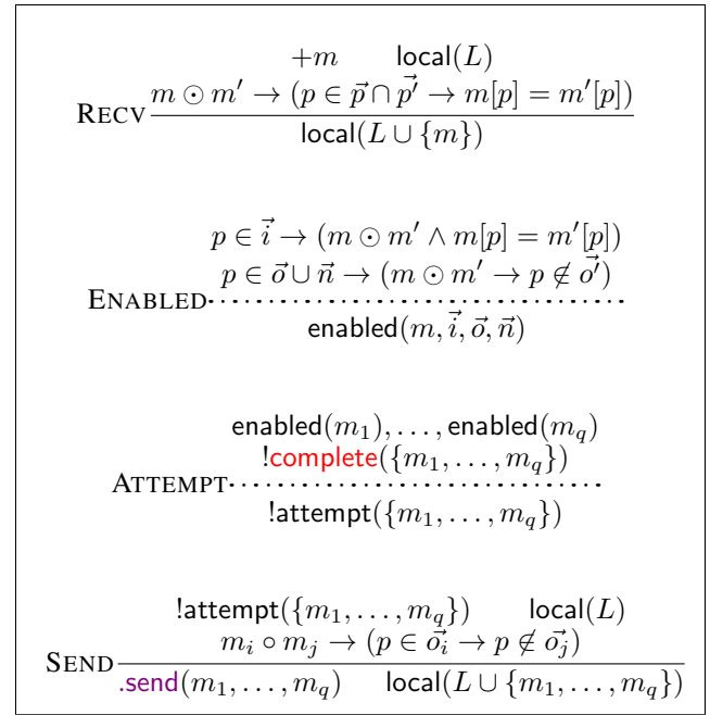
Figure 3: Operational semantics of Orpheus, as inference rules for an agent's state-transition system. Dotted line: inference within a state; solid line: transition from one state to the next. This semantics highlights the modularity of Orpheus. Rules RECV, ENABLED, and SEND are based on the BSPL semantics rendered into Jason, and implemented in our tool. The programmer is responsible only for complete to apply Rule ATTEMPT.
