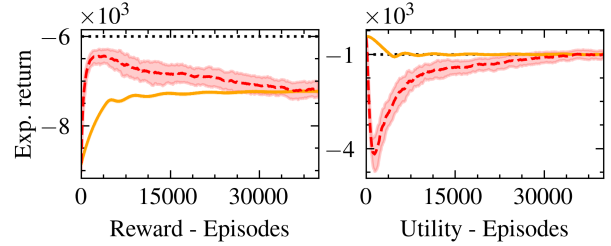
Figure 2: Avg. reward/utility value functions of AD-PGPD (—) and PGDual (- -) iterates in the navigation problem.
