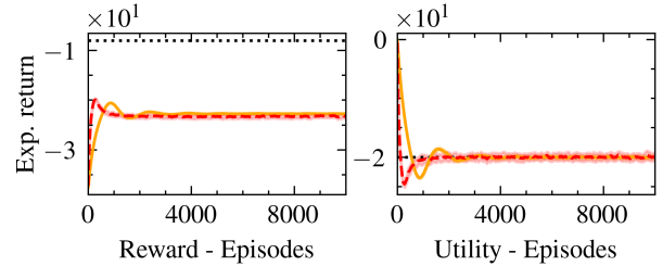
Figure 3: Avg. reward/utility value functions of AD-PGPD (—) and PGDual (- -) iterates in a fluid velocity control.
