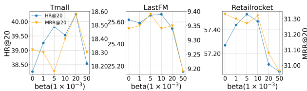
Figure 4: The impact of balance coefficient \beta
