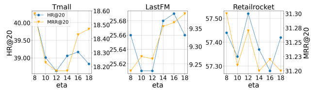
Figure 6: The impact of the hyperparameter \eta
