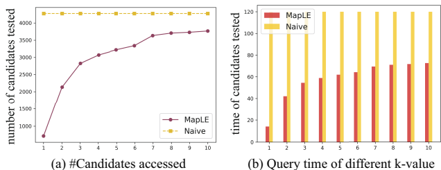
Figure 2: The evaluation result of the MapLE .
