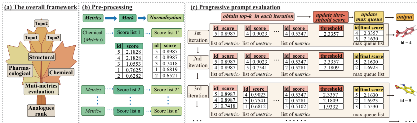
Figure 1: The general framework of MapLE .
