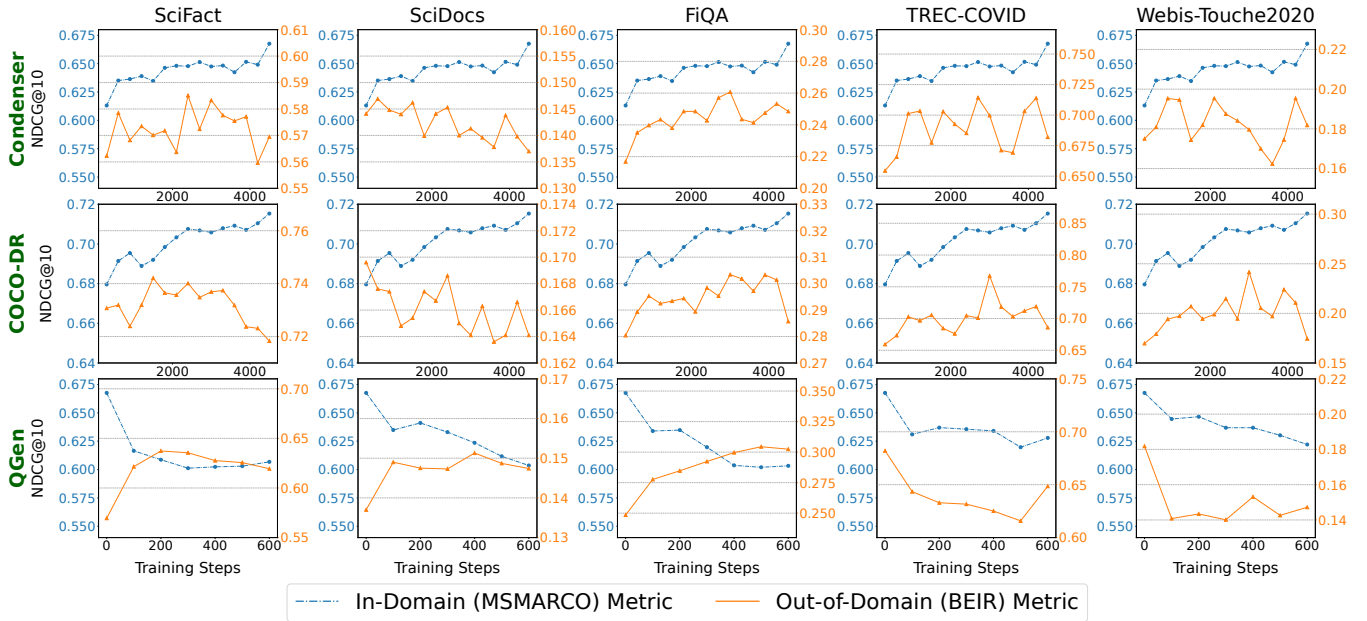
Figure 2: The performance of Condenser, COCO-DR and QGen over different training steps on 5 of BEIR datasets. The blue dotted line indicates the nDCG@10 on MSMARCO (in-domain) and the orange solid line indicates the performance on the corresponding BEIR dataset. The x-axis in the third row is not aligned with the first two rows because QGen uses the target domain generated pseudo data for continuous fine-tuning.
