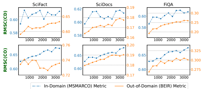
Figure 3: Performance of RMSC(CD) and RMSC(CO) over different training steps on 3 of BEIR datasets. The blue dotted line indicates the nDCG@10 on MSMARCO (in-domain) and the orange solid line indicates the performance on the corresponding BEIR dataset.
