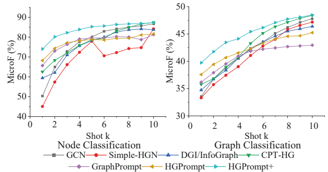
Figure 3: Impact of shots on NC and GC tasks on ACM.
