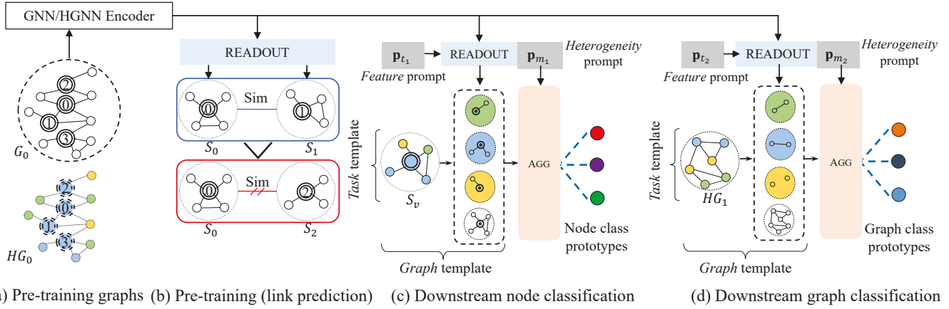
Figure 2: Overall framework of HGPROMPT. (a) Pre-training graphs can be either homogeneous or heterogeneous. (b) Pre-training task with link prediction on a homogeneous graph 1 . (c) Downstream node classification and (d) graph classification on heterogeneous graphs. Black-and-white graphs are homogeneous; colored graphs are heterogeneous, where colors indicate different types of nodes.
