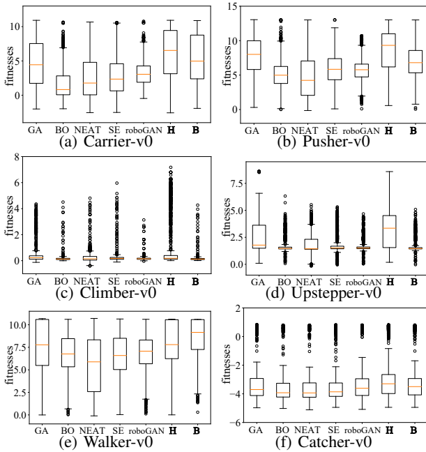
Figure 5: Boxplots of fitness obtained by different methods (H and B stand for MorphVAE-H and MorphVAE-B respectively)
