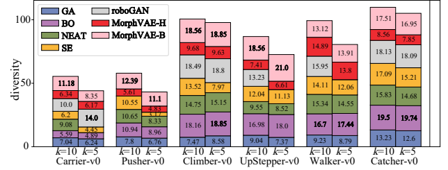
Figure 6: Performance comparison of diversity. In some cases such as roboGAN in Pusher-v0, the algorithm fails to produce more than one robot design that could enter top k percent and thus diversity is not available.
