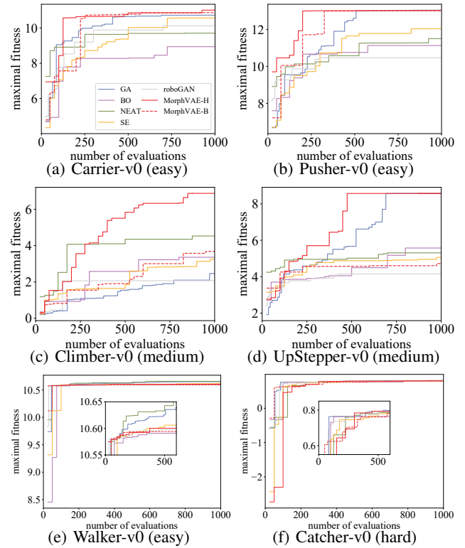
Figure 3: Performance comparison of maximal fitness
