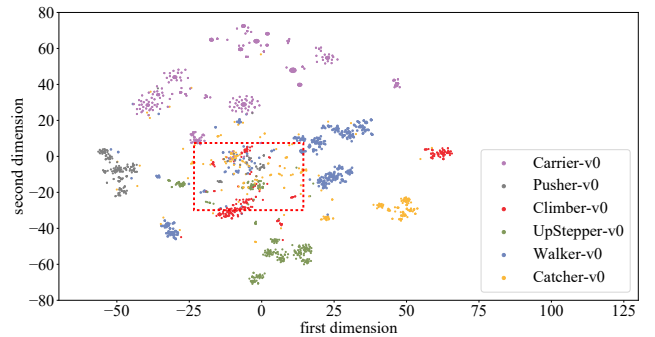
Figure 1: Overlapping of robot designs in multiple tasks
