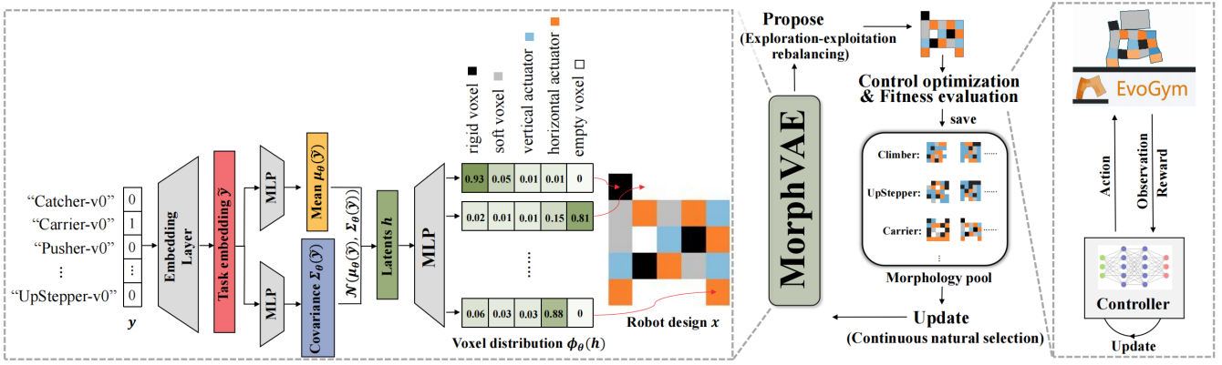
Figure 2: Model architecture and training procedure of MorphVAE. The left dashed box illustrates generative process of MorphVAE, spanning from one-hot tasks encoding to robot design proposals. The circular-flow diagram in the middle outlines the training procedure of MorphVAE. The right dashed box depicts detailed process of a robot to interact with the simulation task, optimize its controller, and ultimately derive its fitness evaluation.
