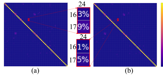
Figure 4: Visualization of classification. The action index is as follows: taking on shoes (16), taking off shoes (17), and kicking something (24). (a) the confusion matrix for CTR-GCN, (b) the confusion matrix for CTR-GCN+NE. It can be observed that, after encoding the semantic information, CTR-GCN+NE can distinguish kicking something from taking on/off shoes more accurately (e.g., errors reduce from 3% and 9% to 1% and 5% respectively).
