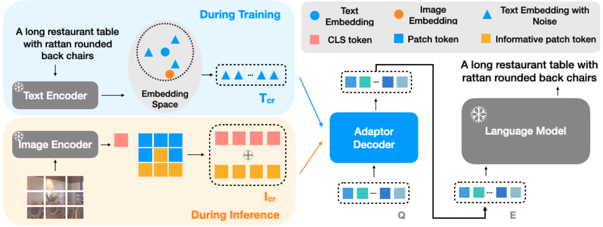
Figure 2: An overview of MacCap pipeline: MacCap learns to generate text based on region noise injected CLIP text feature in text reconstruction training. During inference, MacCap can generate caption without paired data in training. The CLIP and language model are kept frozen in both stages.
