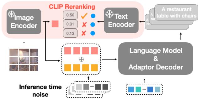
Figure 3: Multiple sampling and filtering pipeline: During inference, each image uses noise to generate several different captions, which are reranked by CLIP to output the best.
