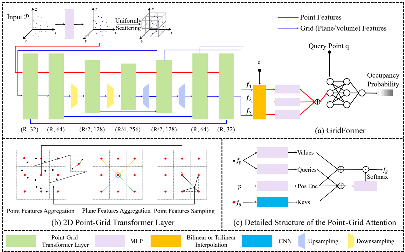
Figure 3: Overview of our method. (a) The architecture of GridFormer. (b) The 2D plane point-grid transformer layer in which the colored arrows represent learnable weights. (c) The detailed structure of the point-grid attention mechanism for point features aggregation. ‘Pos Enc’ denotes position encoding.
