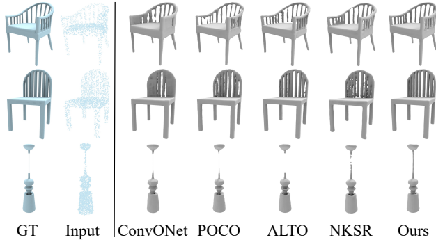
Figure 5: Object-level reconstruction results on the ShapeNet dataset. All the methods are trained and tested on 3000 noisy points.
