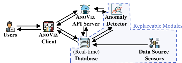
Figure 1: Architectural overview of ANOVIZ.
