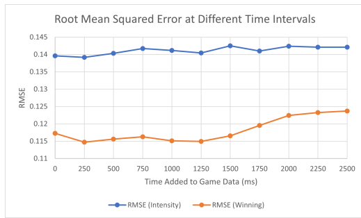
Figure 4: Lagged RMSE values of Bouncy Shots.
