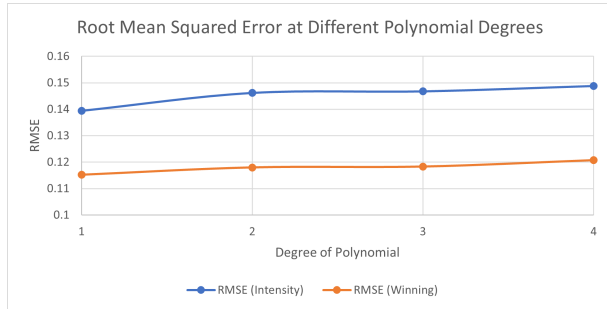
Figure 5: RMSE values of Bouncy Shots varying polynomial degrees.
