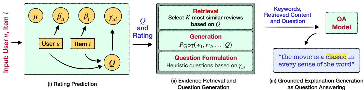
Figure 1: The proposed framework PRAG. Given the input user and item, our model produces a rating estimation (Section ), as well as a latent query Q (Section ). We then use the query to retrieve existing reviews as evidence for the recommendation, and probe a question answering model for natural language explanation (Section ).
