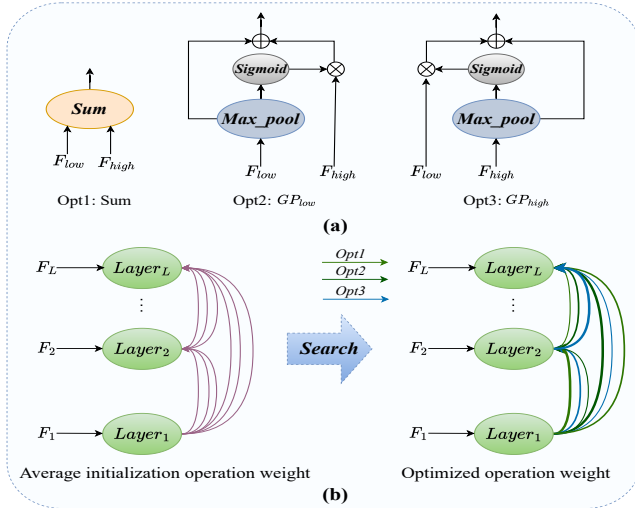
Figure 3: Three feature fusion options, including the sum option and two types of global pooling options, are shown in (a), in which Max_pool denotes max pooling. (b) shows the feature fusion search process. \oplus indicates element-wise summation and \otimes indicates element-wise product.
