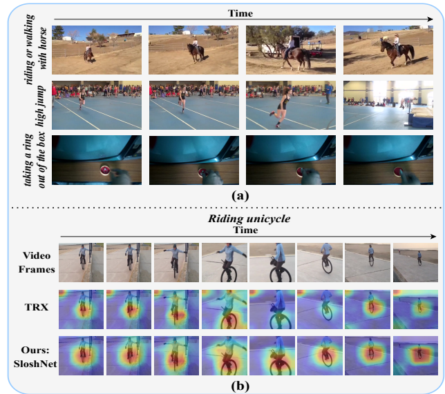
Figure 1: (a): Some examples in few-shot action recognition (b): Visualization of the attention map from the recent work TRX (Perrett et al. 2021) and our proposed SloshNet.
