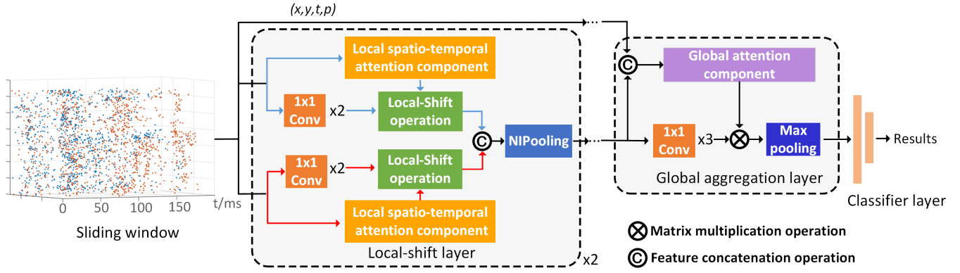
Figure 2: Overview of the proposed LSNet, which contains two local-shift layers, one global aggregation layer and one classifier layer. The local-shift layer extracts multi-scale features for each node and performs the local-shift operation to aggregate features. Blue arrows represent feature extraction and local-shift operation are performed on small receptive field, and red arrows represent large receptive field. The global aggregation layer aims at obtaining high-level global features through global max pooling operation. The classifier layer contains two fully connected layers for predicting results.
