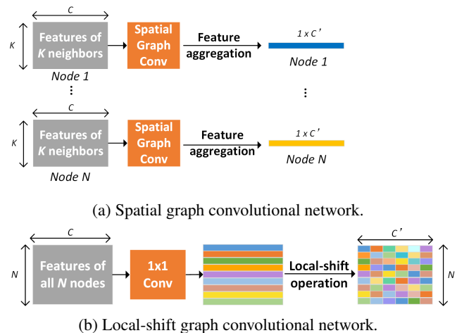
Figure 1: Feature aggregation way of spatial graph convolutional network and local-shift graph convolutional network.
