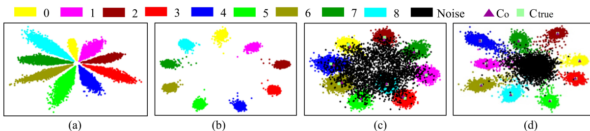
Figure 1: The distribution of deeply learned features under different schemes: (a) softmax loss and clean dataset; (b) joint loss function 1 (softmax loss and centre loss) and clean dataset; (c) joint loss function 1 and noisy dataset; (d) joint loss function 2 ( \mathcal{L} ) and noisy dataset, \lambda = 1 ; C_{os} are updated during the training. C_{true} s are computed by the mean of feature points respectively in each class excluded from noise.
