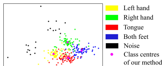
Figure 2: Visualization of feature distribution of subject A07
