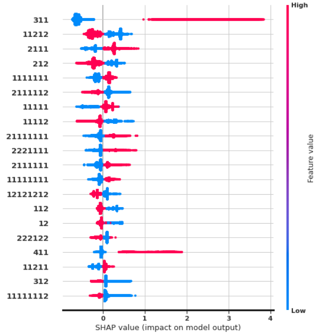
Figure 4: SHAP values of auto-generated features by Seq2Pat . Top-20 features are ranked by importance in descending order. Color indicates high (in red) or low (in blue) feature value. Horizontal location indicates the correlation of the feature value to a high or low model prediction.
