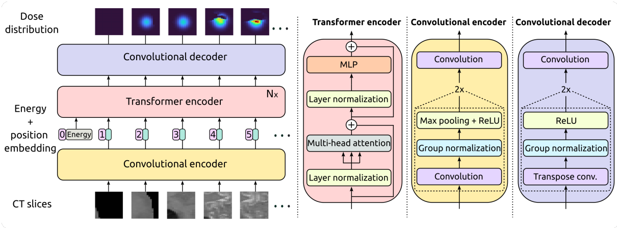
Figure 1: Model architecture. We treat the input and output 3D volumes as a sequence of 2D slices. A convolutional encoder reduces the dimension of the input and extracts important geometrical features. The particle energy is added at the beginning of the resulting sequence. A transformer encoder with causal self-attention then routes information between the encoded input slices. Finally, a convolutional decoder transforms the low-dimensional sequence into an output sequence of 2D dose slices.
