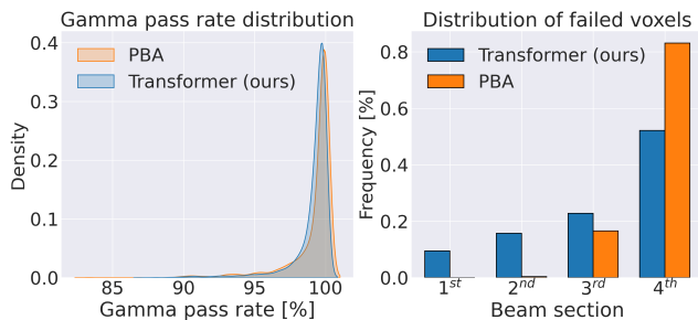
Figure 2: (Left) Distribution of the gamma pass rates across the test set for the PBA and DoTA. (Right) Distribution of the failed voxels along the beam, where each bin shows the ratio between the number of voxels in the test set that fail the gamma evaluation within a section of the beam and the total number of failed voxels.
