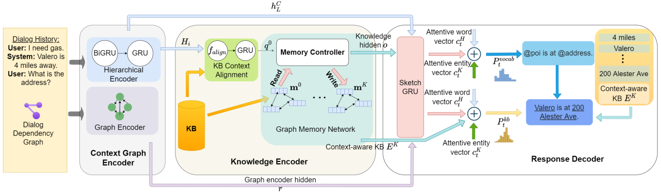
Figure 1: The Framework of our proposed model
