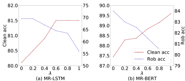
Figure 2: The effect of \lambda on clean accuracy and robustness of accuracy. x -axis is the value of \lambda . Left y -axis is the value of clean accuracy and right y -axis is the value of robustness accuracy.
