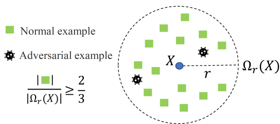
Figure 1: Diagram of Weak Robustness.
