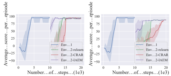
Figure 3: Comparison of IAEM and baselines in Grid-World. Left: The comparison on averaged scores. IAEM can reach the optimal policy in 4000 time-steps while others need at least 6000 time-steps. Middle: The comparison on the transition loss. Optimization of the transition constraint in IAEM is faster than it in other baselines. Right: The ablation study on the invariant action effect. We deactivate the invariant action effect for ablation study, and the result shows that this component contributes to the IAEM sample efficiency.
