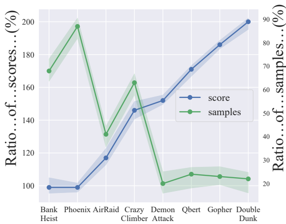
Figure 4: The comparison on scores and samples in Atari games. Blue: The ratio of IAEM to the best baseline on scores. Green: The ratio of IAEM to the best baseline on samples.
