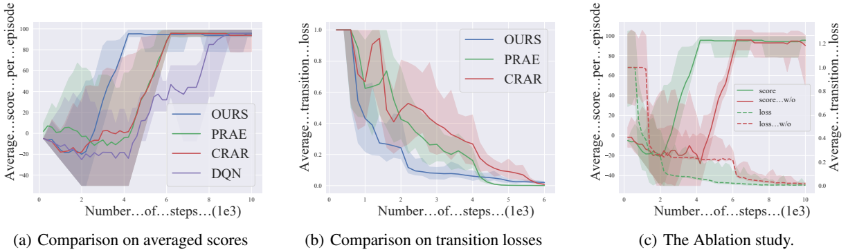
Figure 3: Comparison of IAEM and baselines in Grid-World. Left: The comparison on averaged scores. IAEM can reach the optimal policy in 4000 time-steps while others need at least 6000 time-steps. Middle: The comparison on the transition loss. Optimization of the transition constraint in IAEM is faster than it in other baselines. Right: The ablation study on the invariant action effect. We deactivate the invariant action effect for ablation study, and the result shows that this component contributes to the IAEM sample efficiency.
