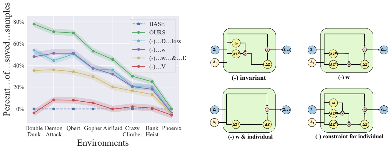
Figure 6: Left: The ablation study for IAEM on sample-efficiency in various Atari games. Right: The architectures of the dynamics deactivating some components. Results show that \omega , the individual action effect and the invariant action effect all contribute to the IAEM sample-efficiency.
