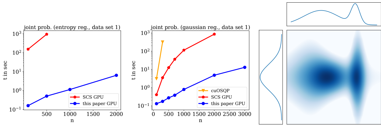
Figure 3: Running times for computing the joint probability distribution from two marginal distributions. The left plot shows the running times when the entropy prior is used and the plot in the middle when a Gaussian prior is used. The right figure visualizes the probabilities.
