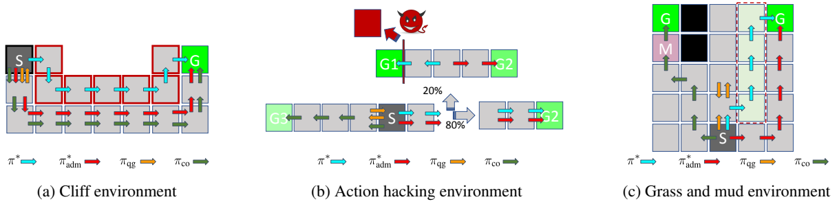
Figure 2. Qualitative assessment : (a) \pi_{co} is the same as \pi_{adm}^* , taking the longer path to the goal state than \pi^* in order to avoid the cliff edge, while \pi_{qg} simply alternates between the starting state and the state below it; (b) \pi_{co} takes the path to the goal state G3—this behavior is less costly to incentivize than navigating to G2 since in the former case the reward designer mainly needs to compensate for the difference in rewards between G3 and G2 (G1 is reachable only 20% of the time from S); (c) \pi^* takes a path through the grass states, \pi_{adm}^* takes a different but admissible path towards the same goal, while \pi_{co} navigates the agent towards the other goal (with a lower cumulative reward, but the corresponding policy is less costly to force). Quantitative assessment : The objective values of (P4-APT) for the approaches based on forcing \pi^* , \pi_{adm}^* , \pi_{qg} , and \pi_{co} are respectively: (a) 0.27, 1.59, 3.93, and 1.59; (b) -2.04 , 14.96, 5.00, and 3.82; and (c) -9.54 , 9.46, 17.26, and 7.92.
