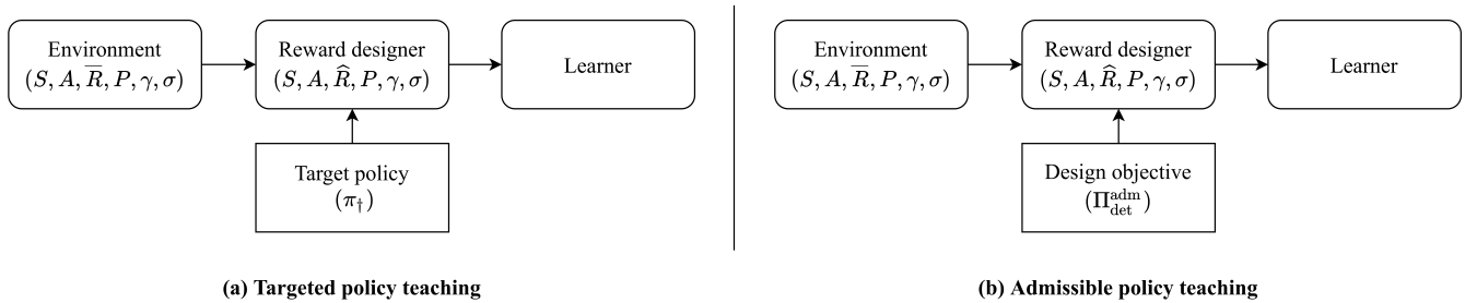
Figure 1. Comparison between targeted and admissible policy teaching. (a) depicts the targeted policy teaching framework. In this framework, the reward designer has a target policy \pi_{\dagger} and perturbs the original reward function \bar{R} to the modified reward function \hat{R} in order to ensure that \pi_{\dagger} is optimal w.r.t \hat{R} . This would ensure that a learner maximizing its performance w.r.t \hat{R} would follow \pi_{\dagger} . Since there may be many suitable \hat{R} , the designer typically chooses the one with minimum modification cost. (b) shows the admissible policy teaching problem studied in this paper. In contrast to a single targeted policy, the designer has a set of admissible policies \Pi_{\text{det}}^{\text{adm}} . The goal of the designer is to modify \bar{R} to ensure that the learner chooses an admissible policy. As before, the designer wants to keep modification cost at a minimum. Unlike the previous setting, we are also interested in the performance of the learner w.r.t the original reward function \bar{R} .
