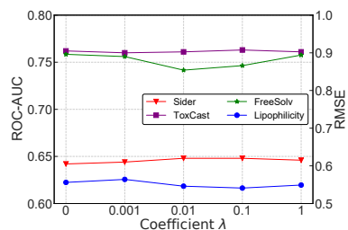
Figure 4: Analysis for the balancing parameter of \mathcal{L}^s .
