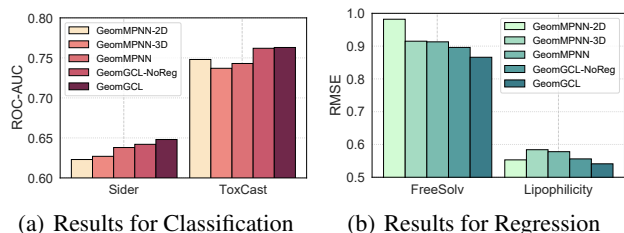
Figure 3: Evaluation of GeomGCL with its variants.
