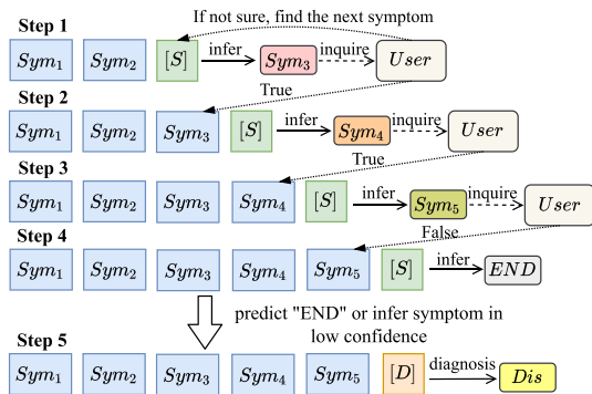
Figure 3: Schematic of inference process.
