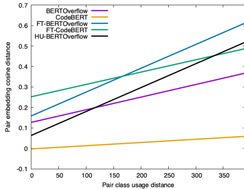
Figure 7: Prediction of embedding distance by class usage (U) similarity for all models. Standard error of regression was less than 1.0e-4 for all models.
