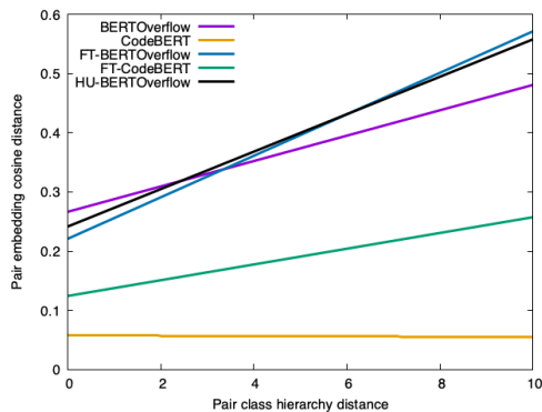
Figure 6: Prediction of embedding distance from class distance (H) for all models. Standard error of regression was less than 0.0002 for all models.
