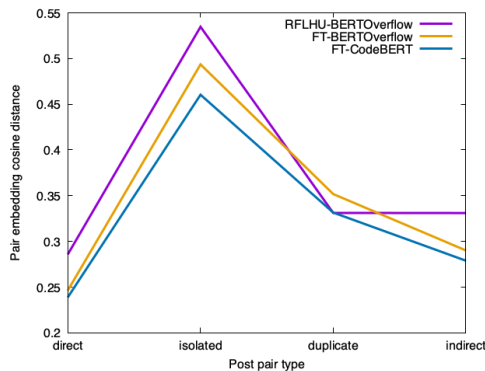
Figure 3: Direct, indirect, duplicate and isolated pair distances models.
