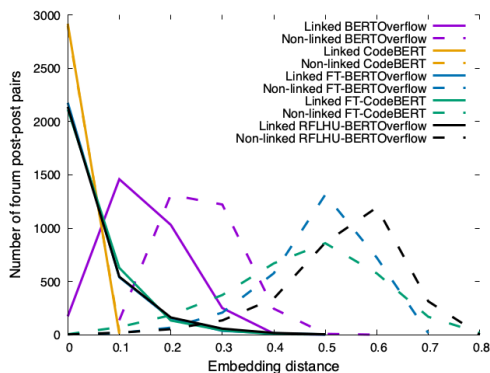
Figure 2: Linked versus unlinked pair distances (L).
