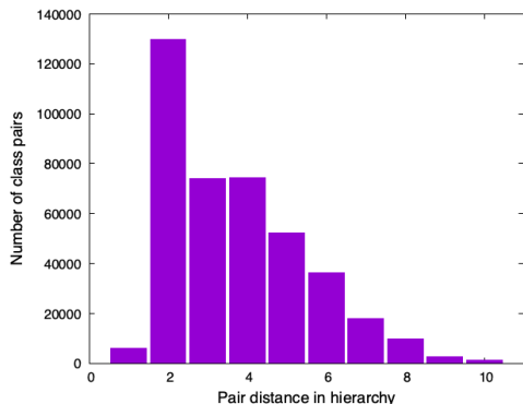
Figure 5: Number of class-pairs by class distance.
