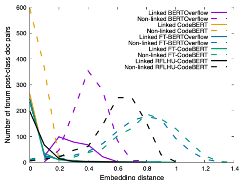
Figure 4: Related and unrelated documentation-post pair distances for some fine-tuned and non-fine-tuned models (F).
