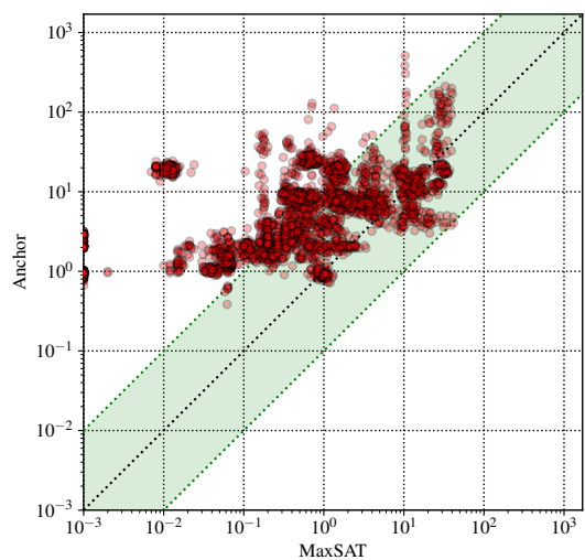
(c) Detailed runtime comparison vs. Anchor
