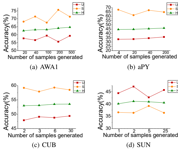
Figure 6: Generating different numbers of diverse features.
