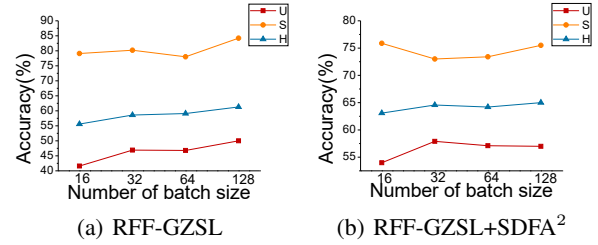
Figure 3: Effects of different batch sizes.
