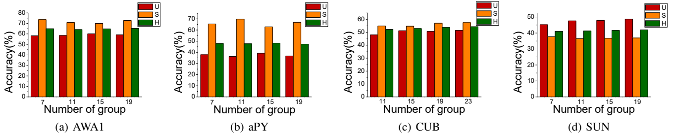
Figure 4: The influence of different grouping numbers on GZSL results in attribute clustering.
