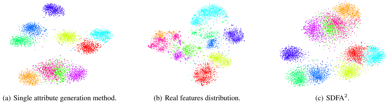
Figure 5: t-SNE graph of visual features generated by single attribute and diversity attribute generation method.
