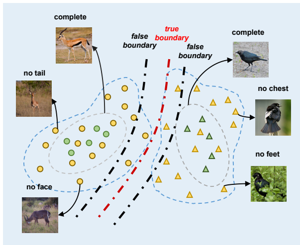
Figure 1: Green represents the generated visual features, and yellow represents the real visual features. Traditional generative methods only use complete and single semantic attributes to generate visual features. This method cannot generate visual features. This makes the distribution of generated features and real features unable to fit. The classification boundary obtained from the visual features generated by single semantic attributes has great fluctuation. There is a big gap with the correct classification boundary.
