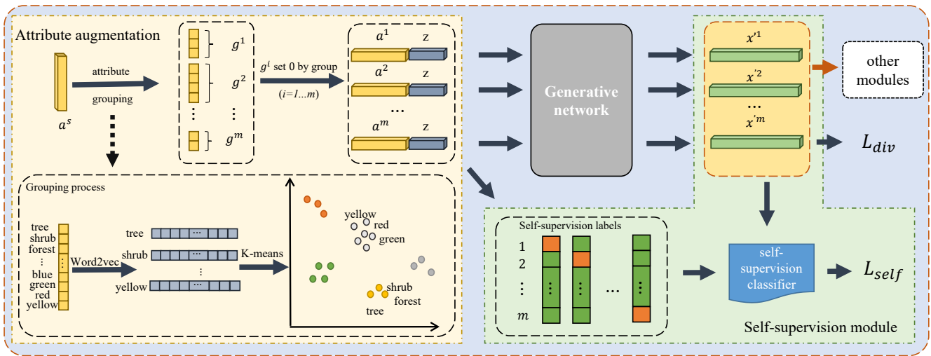
Figure 2: The schematic of SDFFA 2 . We first group attributes, and then make attribute augmentation through setting 0 by group. The obtained attributes are used to generate diversity visual features. The generator and discriminator in generative network are replaceable for different generation networks. Other modules are replaceable network modules that downstream tasks of the generate network. For different GZSL models, other modules are different. At the same time, self-supervision labels are added to the generated visual features for self-supervision classification.
